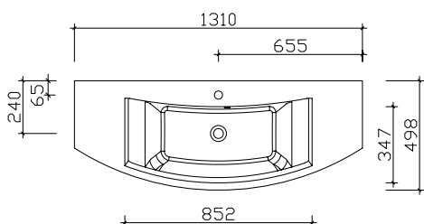
1310 mm BME033M13101
